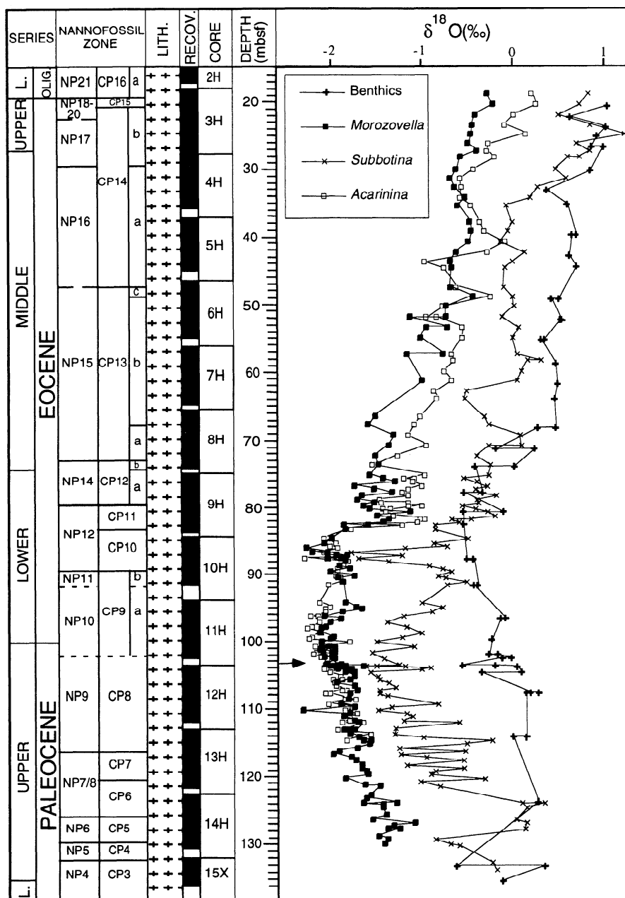
Figure 4. Planktonic and benthic foraminifer \delta^{18}\text{O} (‰ versus Pee Dee belemnite (PDB)) records of the upper Paleocene to upper Eocene of Hole 865B. Planktonic taxa are grouped into genera, and benthic taxa are combined. Calcareous nannofossil zones of Martini [1971] and Bukry [1973, 1975] (using terminology of Okada and Bukry [1980]) are shown at left. Arrow indicates position of benthic foraminiferal extinction.
