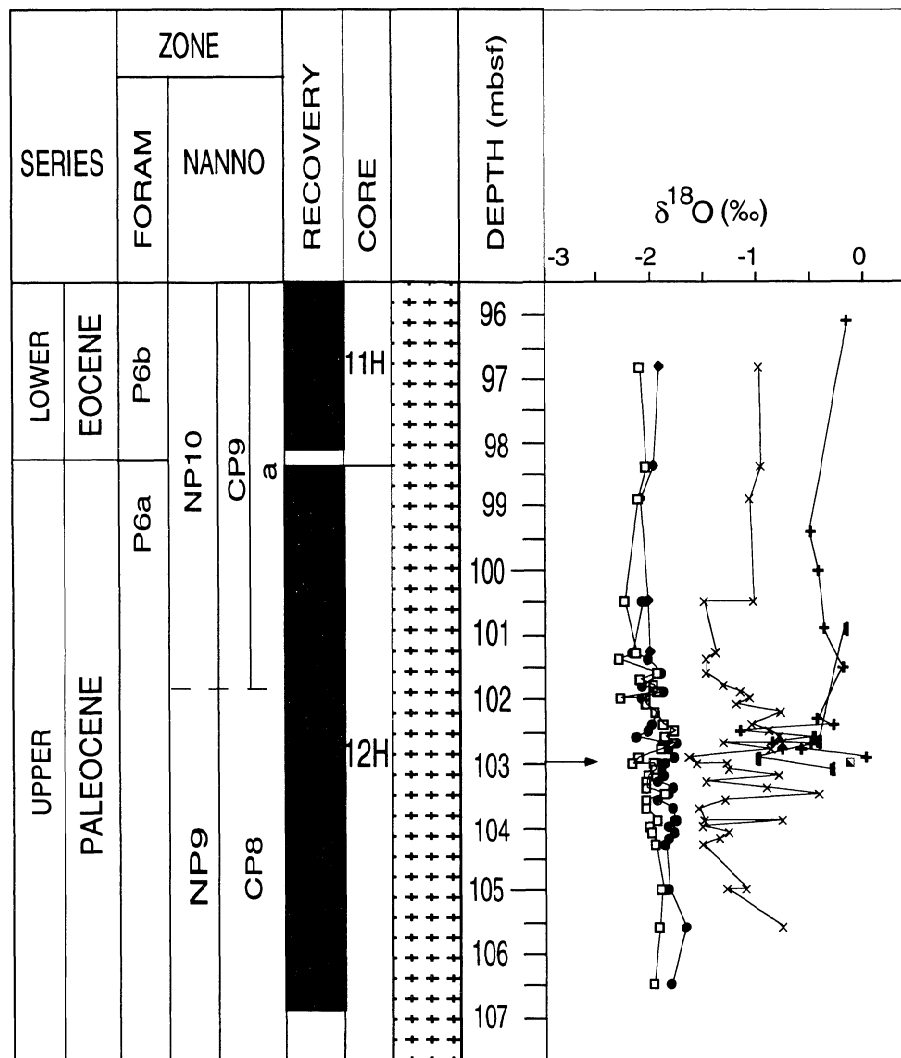
Figure 7. Planktonic and benthic foraminifer \delta^{18}\text{O} (‰ versus PDB) records of the uppermost Paleocene and lowermost Eocene of Hole 865C. Planktonic taxa are separated into species, and benthic taxa are differentiated. See key in Figure 5 for symbols. Calcareous nannofossil zones of Martini [1971] and Bukry [1973, 1975] are shown at left. Planktonic foraminifer subzones of Berggren and Miller [1988] as determined by D. C. Kelly are indicated. Arrow indicates position of benthic foraminiferal extinction.
