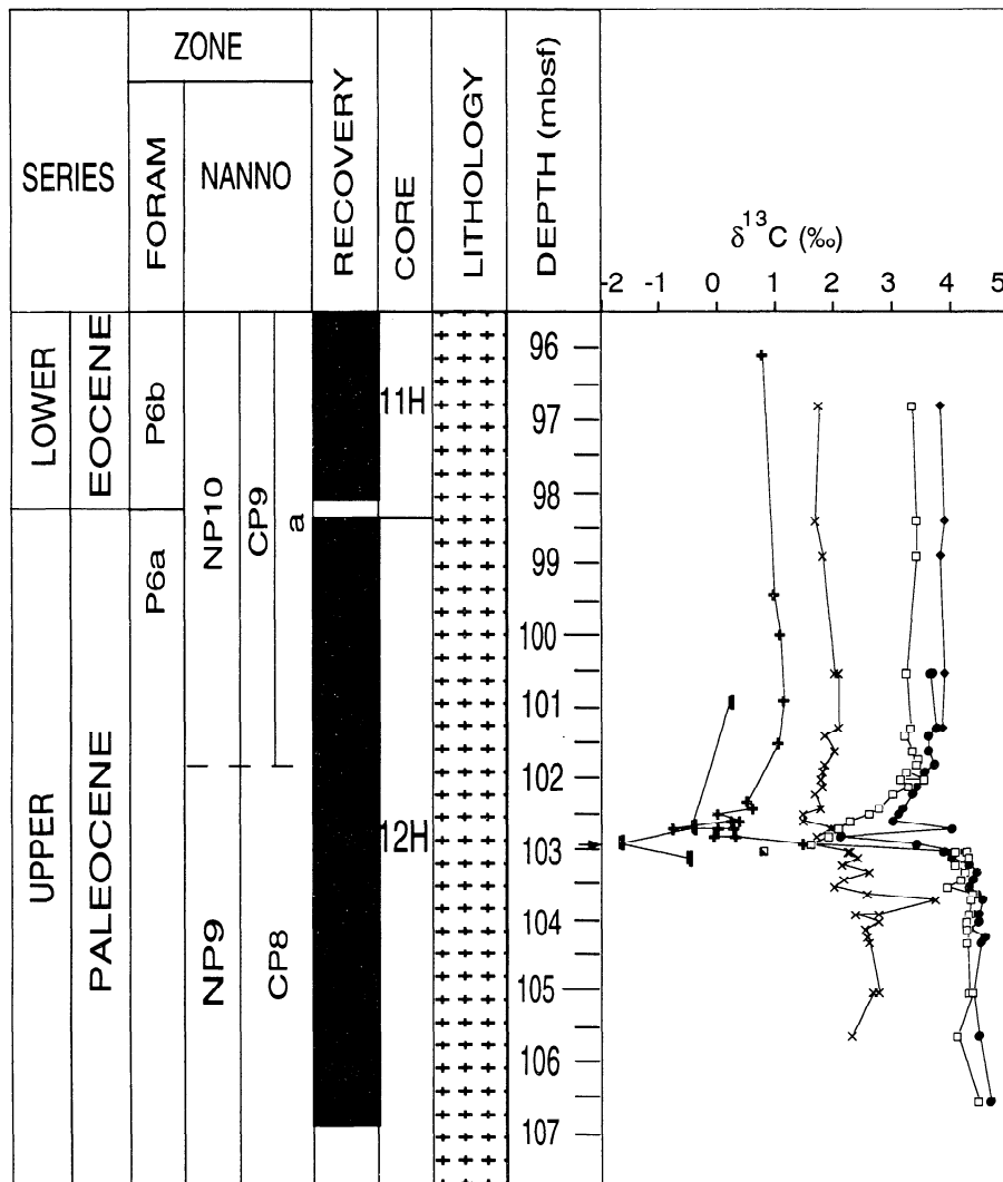
Figure 11. Planktonic and benthic foraminifer \delta^{13}\text{C} (‰ versus PDB) records of the uppermost Paleocene and lowermost Eocene of Hole 865C. Planktonic taxa are separated into species, and benthic taxa are differentiated. See key in Figure 5 for symbols. Calcareous nannofossil zones of Martini [1971] and Bukry [1973, 1975] are shown at left. Planktonic foraminifer subzones of Berggren and Miller [1988] as determined by D. C. Kelly are indicated. Arrow indicates position of benthic foraminiferal extinction.
