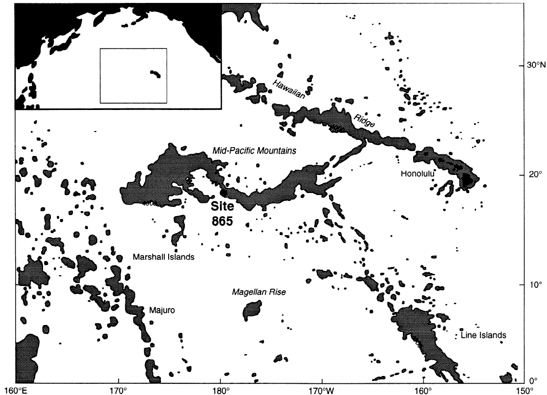
Figure 1. Location of ODP Site 865 on Allison Guyot in the Mid-Pacific Mountains. Inset shows general location of detailed map.
