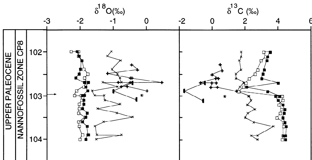
Figure 14. Planktonic and benthic foraminifer \delta^{13}\text{C} and \delta^{18}\text{O} records (‰ versus PDB) of the uppermost Paleocene of Hole 865C. Scale is meters below sea floor. Planktonic taxa are separated into species, and benthic taxa are differentiated. See key in Figure 5 for symbols. Arrow indicates position of benthic foraminiferal extinction.
