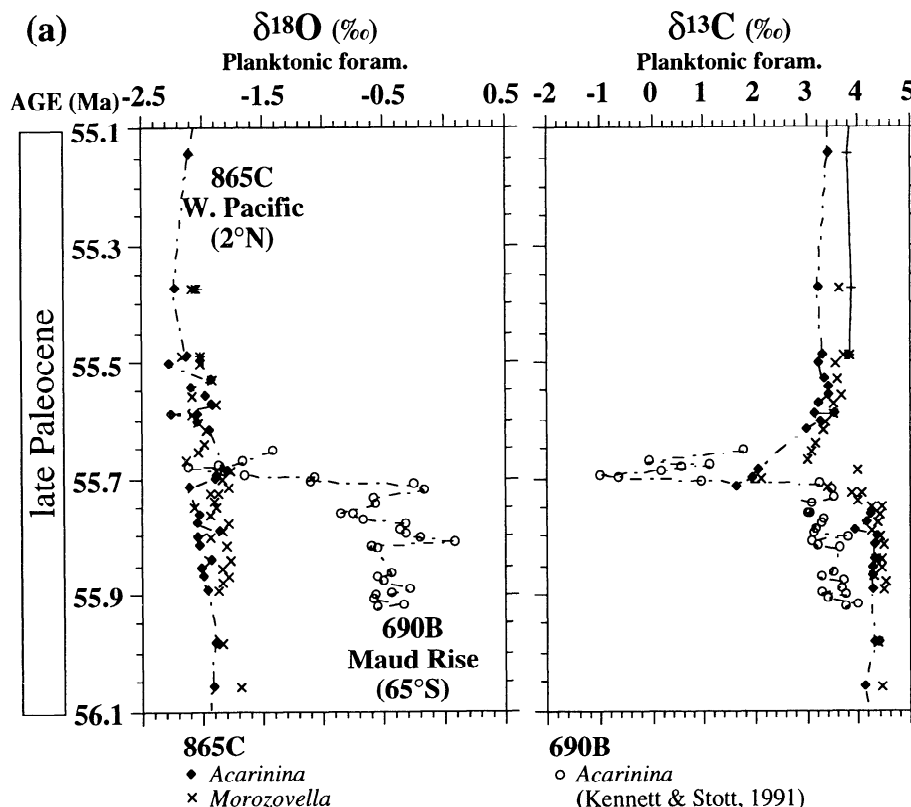
Figure 13. (a) Planktonic and (b) benthic stable isotopic records of the latest Paleocene interval in Hole 865C compared to records from other sites including Site 527 in the South Atlantic [ Thomas and Shackleton , 1995; J. C. Zachos and D. K. Rea, unpublished data, 1994] and Site 690 on Maud Rise [ Kennett and Stott , 1991].
