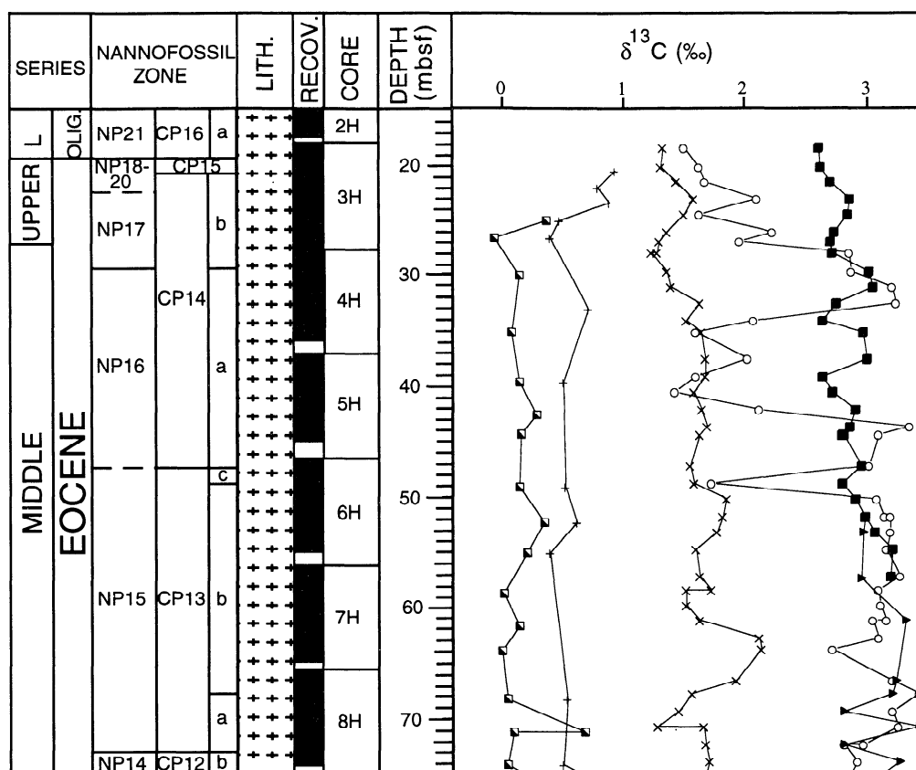
Figure 10. Planktonic and benthic foraminifer \delta^{13}\text{C} (‰ versus PDB) records of the lower to upper Eocene of Hole 865B. Planktonic taxa are separated into species, and benthic taxa are differentiated. See key in Figure 5 for symbols.
