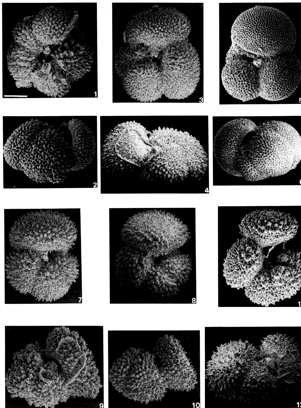
Figure 3. Typical specimens of planktonic foraminifera from Site 865. Specimens 1 and 2 are Acarinina mckannai , specimen 1 is the umbilical view and specimen 2 is the side view; Sample 865C-12H-4, 10-12 cm. Specimens 3 and 4 are A. soldadoensis ; specimen 3 is the umbilical view and specimen 4 is the side view; Sample 865C-10H-4, 60-62 cm. Specimens 5 and 6 are Subbotina spp., specimen 5 is the umbilical view and specimen 6 is the side view; Sample 865B-12H-4, 70-72 cm. Specimens 7-10 are Acarinina spp., specimens 7 and 8 are umbilical views and specimens 9 and 10 are side views; Sample 865B-7H-1, 118-120 cm. Specimens 11 and 12 are Truncorotaloides rohri ; specimen 11 is the umbilical view, specimen 12 is the side view; Sample 865B-5H-5, 50-72 cm. Scale bar represents 100 microns.
