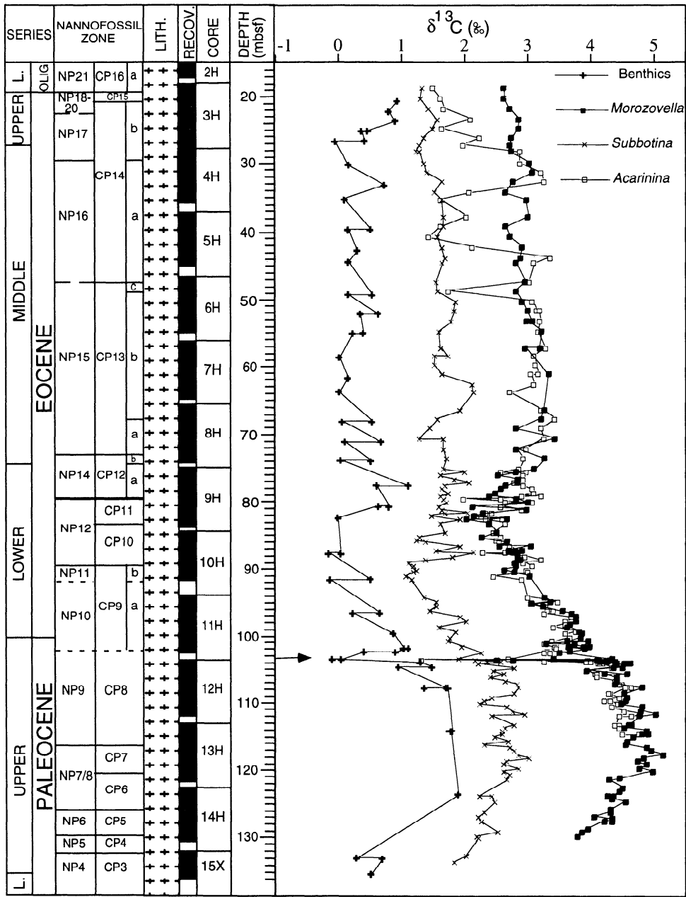
Figure 8. Planktonic and benthic foraminifer \delta^{13}\text{C} (‰ versus PDB) records of the upper Paleocene to upper Eocene of Hole 865B. Planktonic taxa are grouped into genera, and benthic taxa are combined. Calcareous nannofossil zones of Martini [1971] and Bukry [1973, 1975] are shown at left. Arrow indicates position of benthic foraminiferal extinction.
