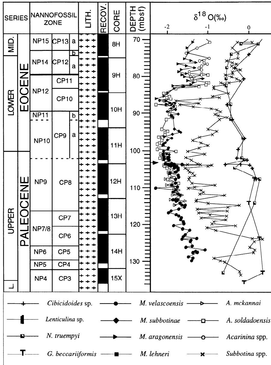
Figure 5. Planktonic and benthic foraminifer \delta^{18}\text{O} (‰ versus PDB) records of the upper Paleocene to lowermost Eocene of Hole 865B. Planktonic taxa are separated into species, and benthic taxa are differentiated. See key below for symbols. Arrow indicates position of benthic foraminiferal extinction.
