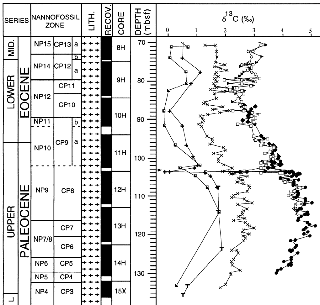
Figure 9. Planktonic and benthic foraminifer \delta^{13}\text{C} (‰ versus PDB) records of the upper Paleocene to lowermost Eocene of Hole 865B. Planktonic taxa are separated into species, and benthic taxa are differentiated. See key in Figure 5 for symbols. Arrow indicates position of benthic foraminiferal extinction.
