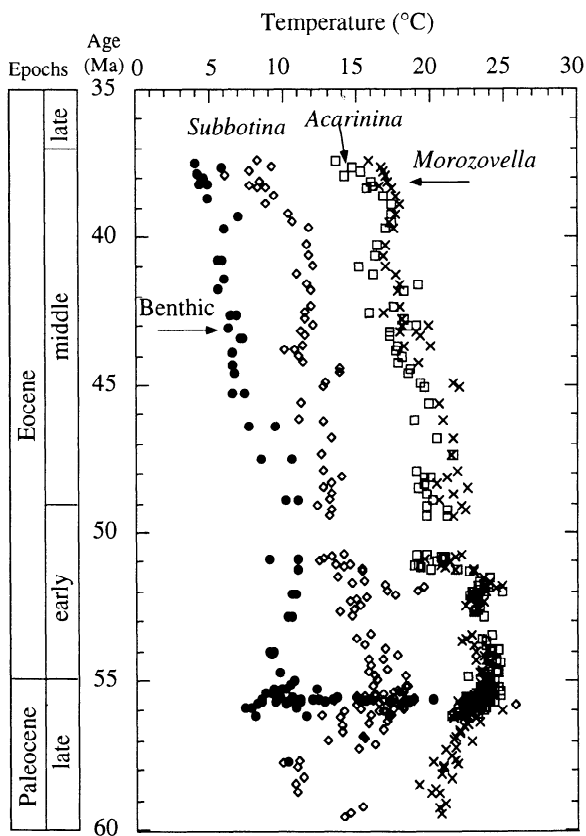
Figure 12. Paleogene paleotemperature history of surface and intermediate waters at Site 865 based on \delta^{18}\text{O} values of planktonic and benthic foraminifera (see text for discussion). Note that temperature scale is inverted relative to other figures.
