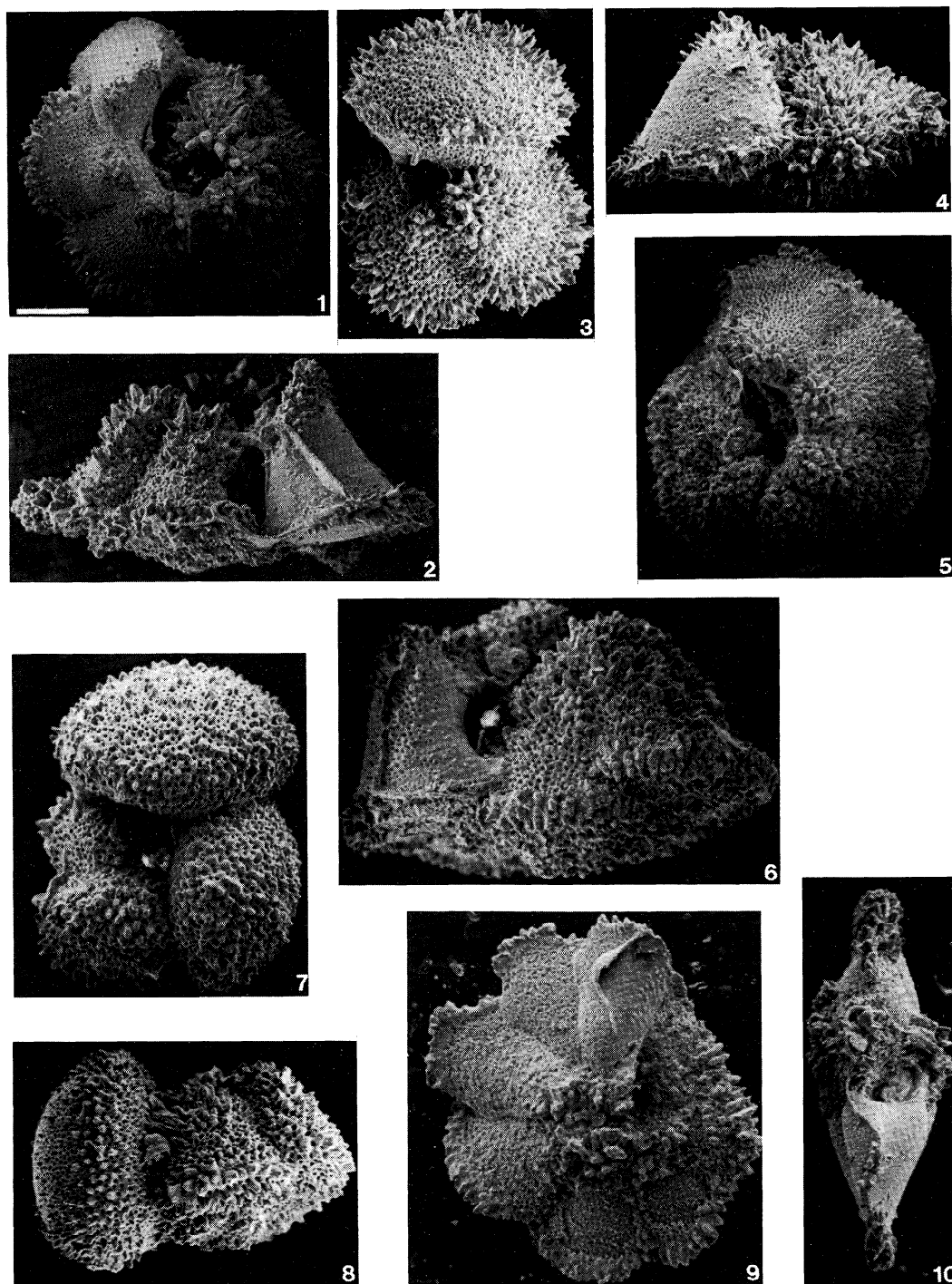
Figure 2. Typical specimens of planktonic foraminifera from Site 865. Specimens 1 and 2 are Morozovella velascoensis , specimen 1 is the umbilical view and specimen 2 is the side view; Sample 865C-12H-4, 10-12 cm. Specimens 3 and 4 are M. subbotinae , specimen 3 is the umbilical view and specimen 4 is the side view; Sample 865C-12H-4, 10-12 cm. Specimens 5 and 6 are M. aragonensis ; specimen 5 is the umbilical view and specimen 6 is the side view; Sample 865B-10H-2, 4-6 cm. Specimens 7 and 8 are M. quetra , specimen 7 is the umbilical view and specimen 8 is the side view; Sample 865B-10H-2, 60-62 cm. Specimens 9 and 10 are M. lehneri , specimen 9 is the umbilical view and specimen 10 is the side view; Sample 865B-4H-6, 20-22 cm. Scale bar represents 100 microns.
